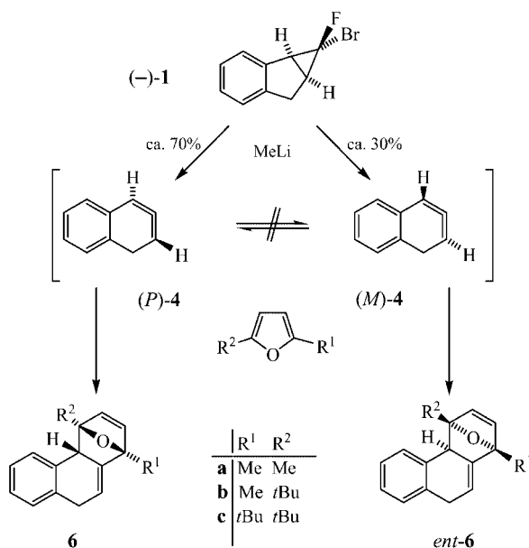
Scheme 3. Generation of the isonaphthalene 4 from the pure enantiomer (1 R ,1 aS ,6 bS )- 1 [( - )- 1 ] and interception of 4 by 2,5-disubstituted furans.
